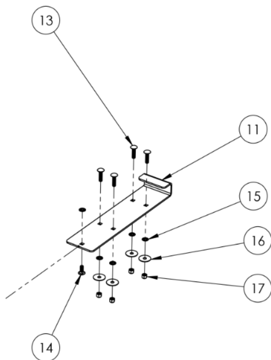
(Fig. 5) Assemble the Mounting Bracket's fasteners as shown here.
