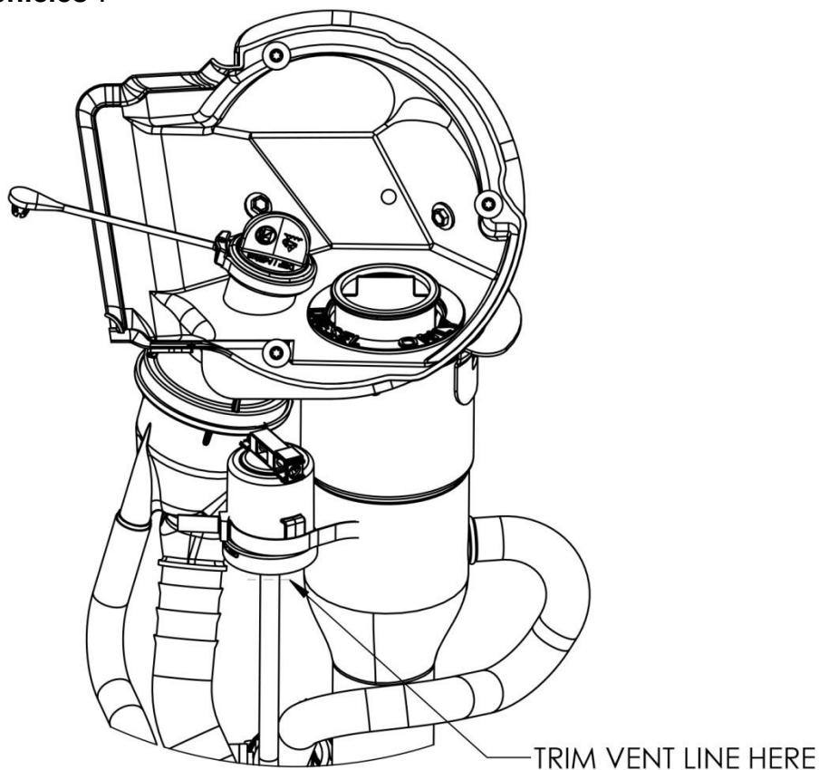
(Fig. 20) Fill spout assembly on some Chrysler RAM products. The vent line breather is shown just above the point of the arrow. Since the vehicle's underbody tank is now also vented through the Travel Trekker™, the vent line can be cut where indicated on the illustration. Then, slip on a short piece of 3/8" hose over the vent line and plug with a plastic plug, or small cap screw, etc. Be sure to use hose clamps to insure a leak-proof seal.
