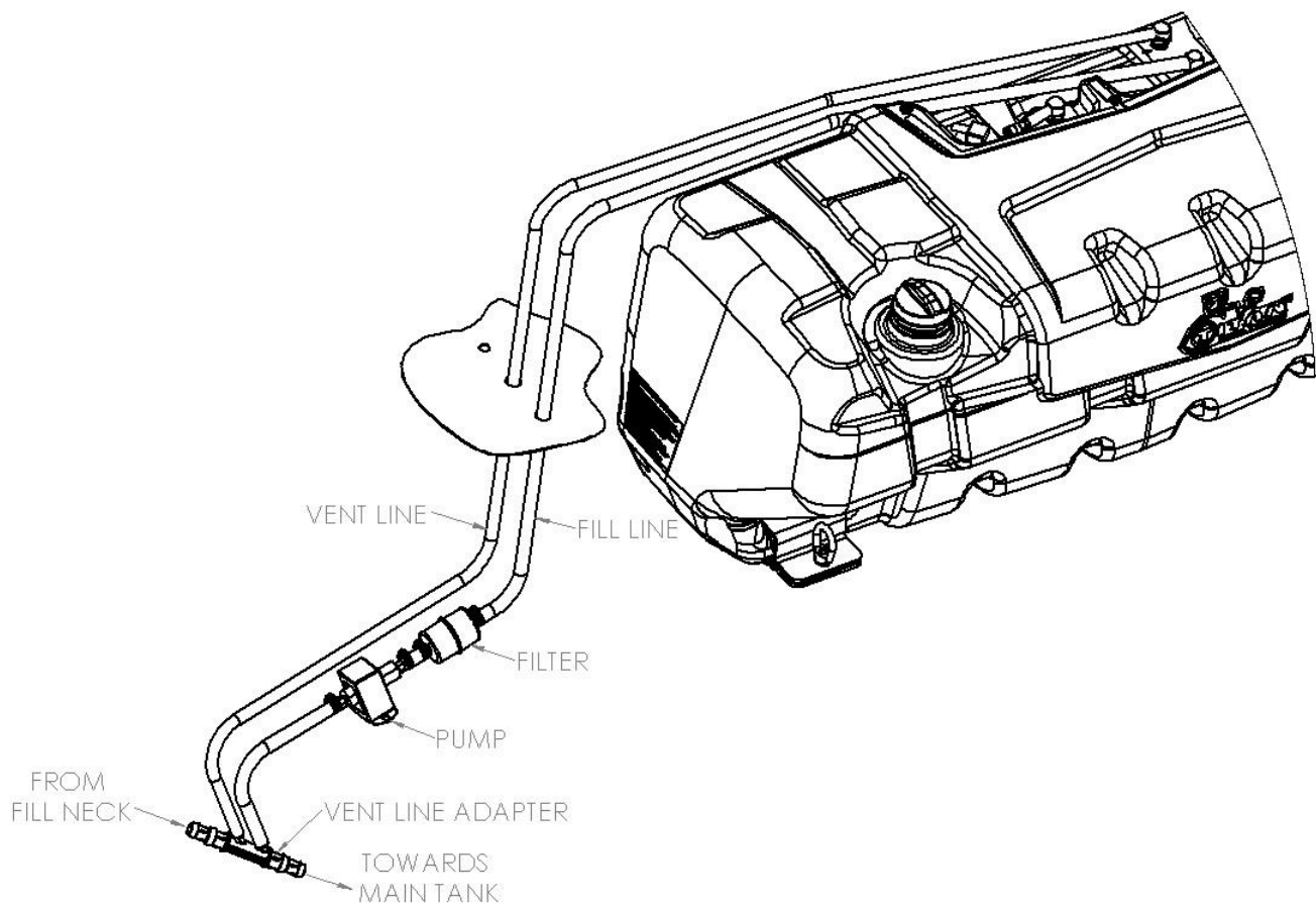
(Fig. 12) Plumbing Diagram for Model 5410040 Travel Trekker™, 40 gallon with TITAN™ pump system.
