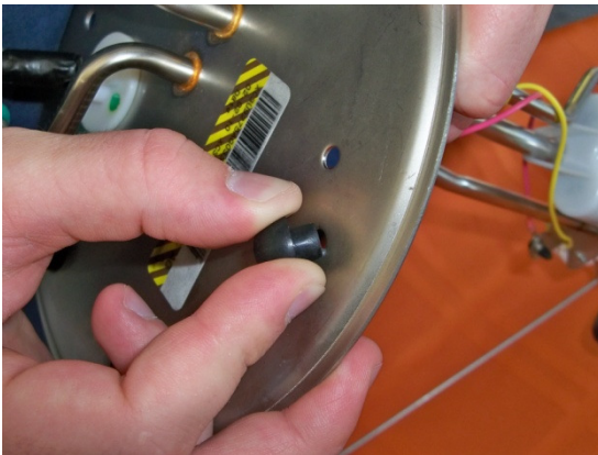
(Fig. 3) Work plug into the hole.
