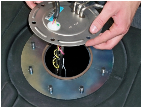
(Fig. 11) Place sending unit on top of "O" ring.
